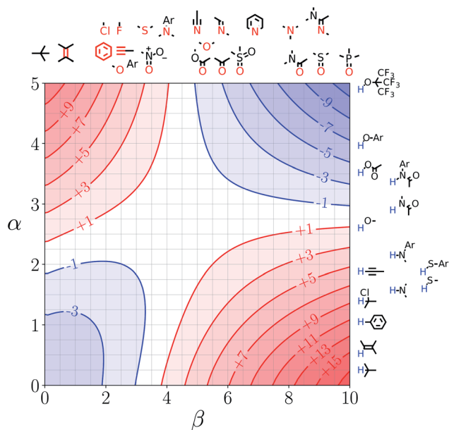
Fig. 4 FGIP for the interaction of two solutes in water at 298 K ( \Delta\Delta G_{FGI} in \text{kJ mol}^{-1} ). The solute–solute interactions are favourable in the blue region, and unfavourable in the red region.
