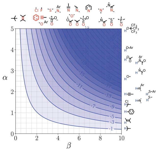
Fig. 3 FGIP for the interaction of two solutes in a hypothetical room temperature liquid state of a noble gas where the concentration of solvent SSIPs is 160 M ( \Delta\Delta G_{FGI} in \text{kJ mol}^{-1} ).
