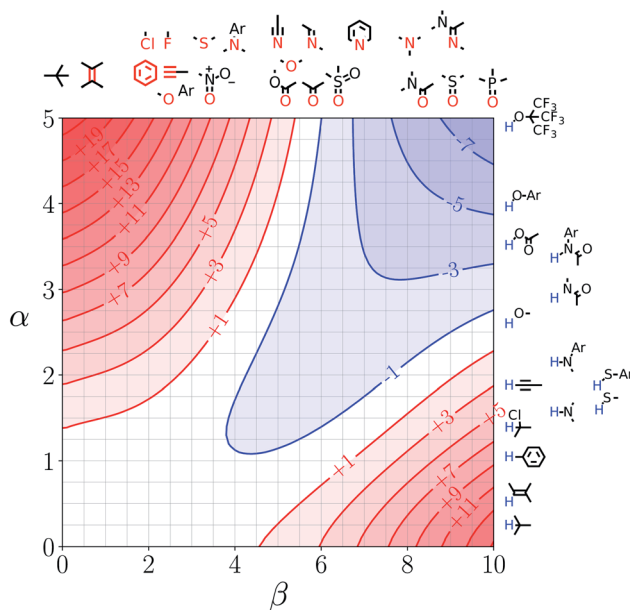
Fig. 5 FGIP for the interaction of two solutes in ethanol at 298 K ( \Delta\Delta G_{FGI} in \text{kJ mol}^{-1} ). The solute–solute interactions are favourable in the blue region, and unfavourable in the red region.
