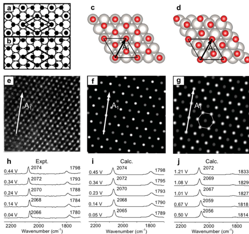
Fig. 1 Pt(111)( 2 \times 2 )-3CO adstructures at 0.04–0.44 V vs. SHE in a CO-saturated 0.1 M \text{HClO}_4 aqueous solution: (a and b) the two possible adstructures ( 2 \times 2 )-3CO \alpha_1 and \alpha_2 , respectively, proposed by Villegas et al. ; (c and d) the respective optimized structures; (e) the measured EC-STM pattern; 44 (f and g) the corresponding calculated patterns of the \alpha_1 and \alpha_2 structures; (h) the measured EC-IR spectra; 47 and (i and j) the corresponding calculated spectra of the \alpha_1 and \alpha_2 adstructures. Images (a), (b) and (e) adapted from ref. 44 with permission, copyright (1994) American Institute of Physics; image (h) adapted from ref. 47 with permission, copyright (2000) American Chemical Society.
