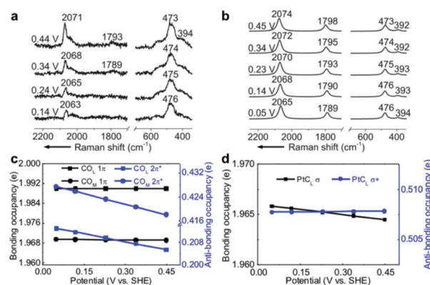
Fig. 2 (a) Experimental EC-Raman spectra of a Pt(111) single-crystal electrode measured by SHINERS at 0.14–0.44 V vs. SHE in a CO-saturated 0.1 M \text{HClO}_4 aqueous solution. (b) Calculated EC-Raman spectra of the ( 2 \times 2 )-3CO \alpha_1 adstructure. Potential-dependent NBO occupancies of the (c) 1\pi and 2\pi^* orbitals of the \text{CO}_L and \text{CO}_M bonds and the (d) \sigma and \sigma^* orbitals of the \text{PtC}_L bond. The slopes of the NBO occupancies are listed in Table S1 † . The detailed NBO wavefunctions are listed in Fig. S6 and S7 † .
