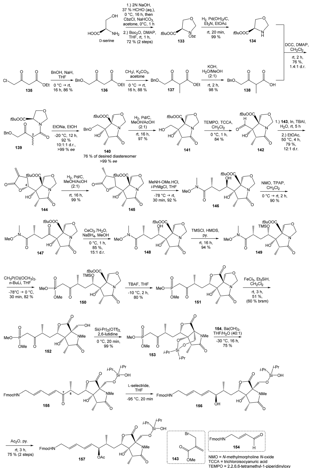
Scheme 11 Synthesis of the right-hand and middle fragment derivative 157 of neoxazolomycin by Kim.
