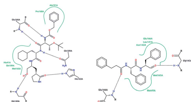
Fig. 3 2-D interaction profiles of TG0205221 (2GX4.pdb) and Cm -FF-H (3SN8.pdb) with active site residues of SARS-CoV-1 3CLpro; hydrogen bonds are shown as broken lines, and hydrophobic interactions are shown in green. The picture was prepared using the "poseview" tool.
