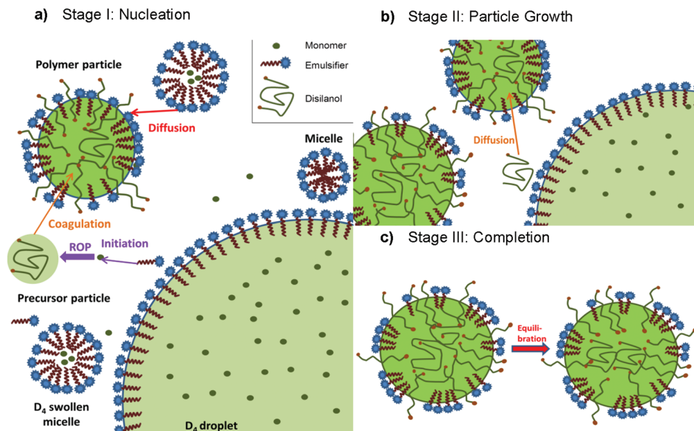
Scheme 11 Schematic presentation of the three stages of emulsion polymerization of cyclic siloxanes (exemplary for D 4 ). 125,126
