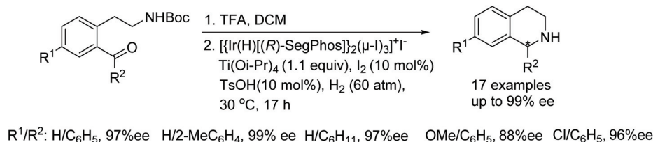
Fig. 3 Reductions of 1-aryl-3,4-dihydroisoquinolines and enantioselective synthesis of Solifenacin.
