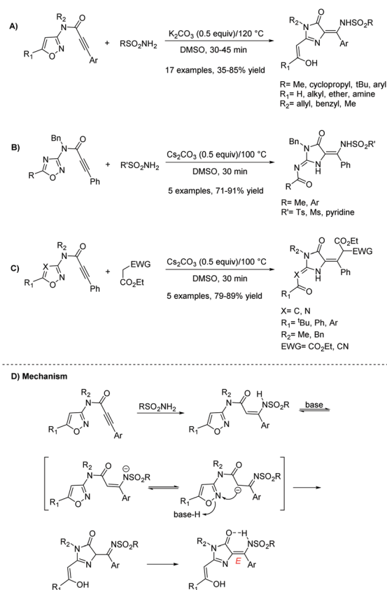
Scheme 28 Cai and co-workers' synthesis of imidazol-4-ones via rearrangement of isoxazoles.
