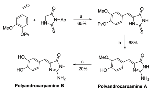
Scheme 45 The first total synthesis of polyandrocarpine A and B. Reagents (a) \text{NaOAc} , \text{AcOH} , reflux, 2 h; (b) TBHP (15 equiv.), aq. \text{NH}_4\text{OH} , \text{MeOH} , rt, 72 h; (c) \text{BBr}_3\text{-SMe}_2 , DCE, reflux, 15 min.
