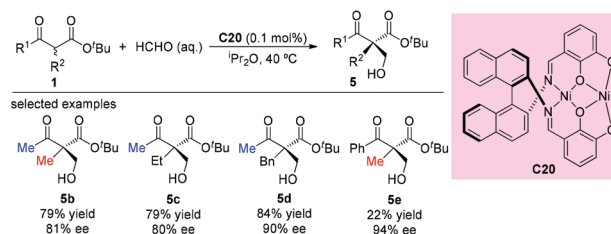
Scheme 29 Ni 2 -Schiff base catalyzed aldol reaction of β-ketoesters with HCHO.
