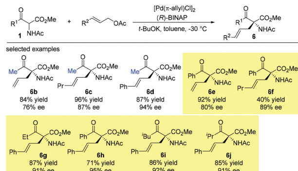
Scheme 31 Asymmetric allylation of α-acetamido-β-ketoesters.
