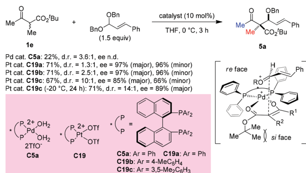
Scheme 28 Aldol reaction of an acyclic β-ketoester with Pt-complex catalysis.
