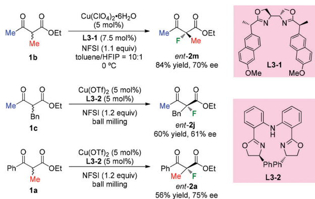
Scheme 7 Copper-catalyzed enantioselective α-fluorination of β-ketoesters.
