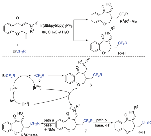
Scheme 5 The synthesis of \text{CF}_2 -containing benzoxepine derivatives.
