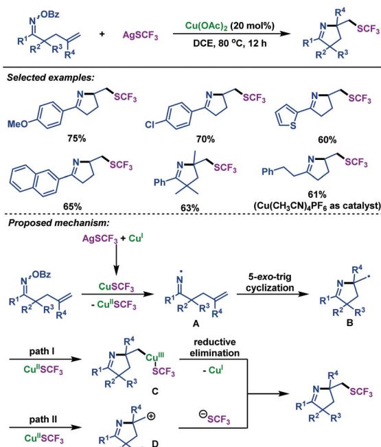
Scheme 7 Zhu's copper-catalyzed imino-trifluoromethylthiolation of \gamma,\delta -unsaturated oxime esters with AgSCF 3 .
