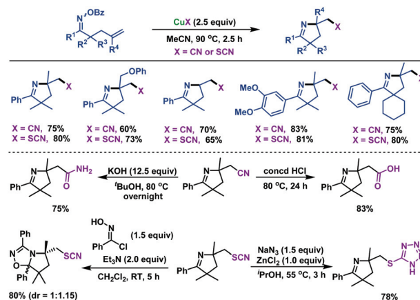
Scheme 9 Zhu and Chen's CuX (X = CN or SCN) promoted imino-cyanogenation and imino-thiocyanation of \gamma,\delta -unsaturated oxime esters.
