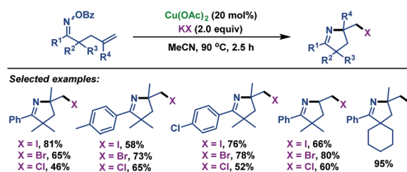
Scheme 10 Zhu and Chen's copper-catalyzed imino-halogenation of \gamma,\delta -unsaturated oxime esters with KX.
