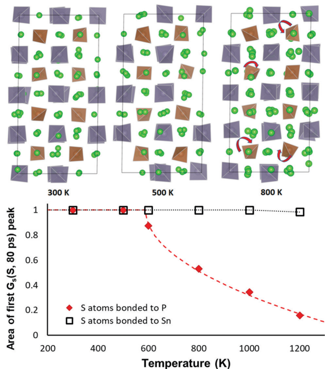
Fig. 9 Effect of temperature on the tetrahedral orientation in \text{Na}_{11}\text{Sn}_2\text{P}_{12}\text{S}_{12} . Top row: Structure models at the end of the 80 ps AIMD simulations for three selected temperatures. Up to 500 K the orientation of the \text{PS}_4 and \text{SnS}_4 remains essentially unchanged over the runtime of the AIMD simulations, while at 800 K the brown \text{PS}_4 tetrahedra become rotationally disordered, whereas the orientation of the grey \text{SnS}_4 remains unchanged. Bottom: Area A_{\text{rel}} under the first peak ( r < 1.8 \text{ \AA} ) of the self-part of the van Hove correlation function G_S(S, 80 \text{ ps}) at a given temperature T over the 80 ps runtime of the AIMD simulations relative to the area at T = 300 \text{ K} . Open squares refer to S atoms of \text{SnS}_4 groups and clarify that the orientation of the \text{SnS}_4 remains unchanged up to at least 1000 K. The filled red diamonds refer to S atoms of \text{PS}_4 groups and reveal an orientational order–disorder phase transition. The broken red line represents a fit to the data according to the function A_{\text{rel}}(T > T_0) = 1 - \text{const.} \times (T - T_0)^{0.5} .
