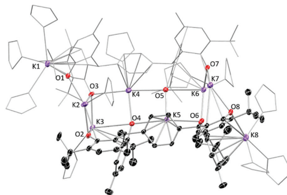
Fig. 1 Solid-state structure of complex \mathbf{1}^{\text{Me}} . Thermal ellipsoids of non-carbon atoms are shown at 30% probability. All hydrogen atoms and lattice solvent molecules are omitted for clarity.
