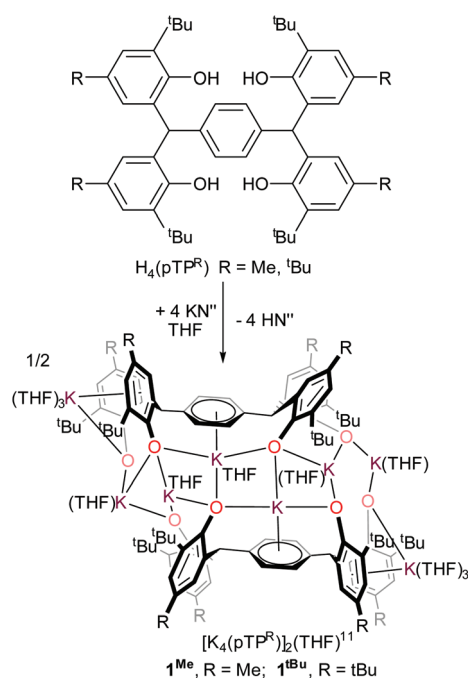
Scheme 1 Synthesis of tetrapotassium salt \mathbf{1}^{\text{R}} .
