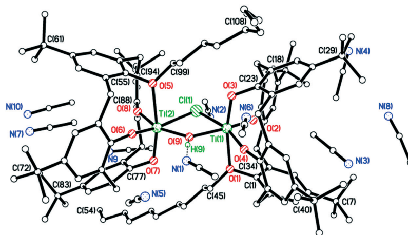
Fig. 7 Molecular structure of [\text{Ti}(\text{O})_3(\text{On-decyl})]_2(\mu\text{-Cl})(\mu\text{-OH}) \cdot 8.5\text{MeCN} ( 10 ·8.5MeCN) (most H atoms are omitted for clarity). Selected bond lengths (Å) and angles (°): Ti(1)–O(1) 2.381(3), Ti(1)–O(2) 1.817(3), Ti(1)–O(3) 1.852(3), Ti(1)–O(4) 1.793(3), Ti(1)–O(9) 2.000(3), Ti(1)–Cl(1) 2.5177(14); O(1)–Ti(1)–O(3) 168.54(13), O(2)–Ti(1)–O(4) 102.84(15), Cl(1)–Ti(1)–O(9) 74.82(10), Ti(1)–O(1)–C(1) 112.8(2), Ti(1)–O(2)–C(12) 150.5(3), Ti(1)–O(3)–C(23) 119.9(2), Ti(1)–O(4)–C(34) 168.3(3).
