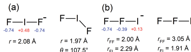
Fig. 2 Calculated equilibrium geometries at the CCSD(T)//def2-TZVPD level of theory for: (a) [\text{F}-\text{I}-\text{F}]^- and [\text{F}-\text{I}-\text{F}] , and (b) [\text{F}-\text{F}-\text{I}]^- and [\text{F}-\text{F}-\text{I}] . NBO charges (red and blue font) are given for the anions. The lowest energy isomer, [\text{F}-\text{I}-\text{F}]^- has D_{\infty h} symmetry, and [\text{F}-\text{I}-\text{F}] has C_{2v} symmetry.
