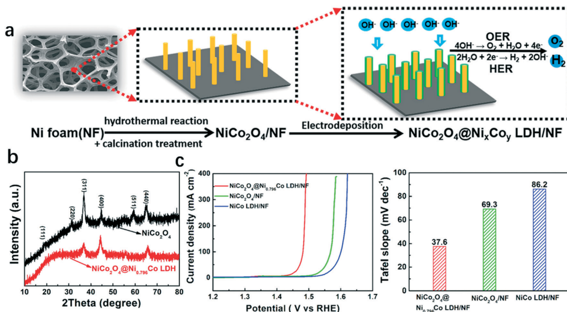
Fig. 2 Hybrid catalyst NiCo 2 O 4 @Ni 0.796 Co LDH/NF with amorphous Ni 0.796 Co LDH and crystallized NiCo 2 O 4 as the shell and core, respectively. 37 (a) Illustration of the fabrication process of the hybrid catalyst, (b) XRD of NiCo 2 O 4 and NiCo 2 O 4 @Ni 0.796 Co LDH; (c) polarization curves and Tafel slopes of NiCo 2 O 4 @Ni 0.796 Co LDH/NF, NiCo LDH/NF, and NiCo 2 O 4 /NF.
