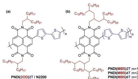
Scheme 1 (a) Structure of PNDI(2OD)2T . (b) Structures of target compounds with 4-decyl-2-(2-decyl(tetradecyl)hexadecyl) chains as multibranching aliphatic side chains (MBS) and up to six unsubstituted thiophene units.
