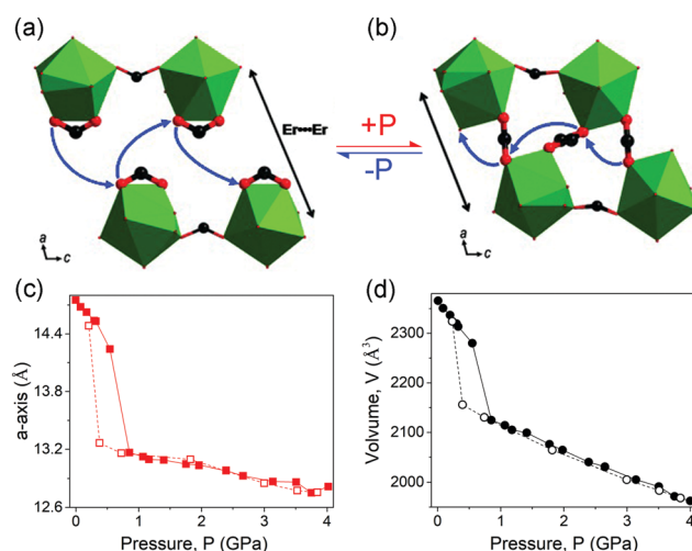
Fig. 19 Partial crystal structure changes of the [tmenH_2][Er(HCOO)_4]_2 before (a) and after (b) compression. Lattice parameter changes of a (c) and volume (d). The data collected with increasing and decreasing pressure are plotted with filled and empty spheres, respectively. Reprinted with permission from ref. 124.
