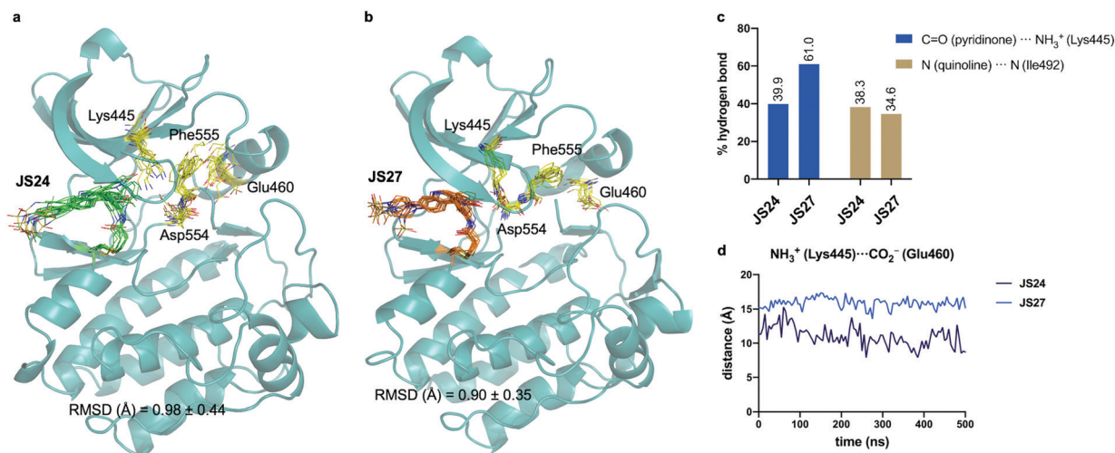
Fig. 4 (a and b) Structural ensembles derived from 0.5 \mu\text{s} MD simulations on BMX covalently linked to JS24 and JS27 . (c) Population of the most relevant hydrogen bonds between the ligands and BMX derived from the MD simulations. (d) Evolution of the Lys445–Glu460 distance along the MD simulations of both complexes. See also Videos 1 and 2 (ESI†). JS24 , JS27 , Lys445, Glu460, Asp554 and Phe555 are shown as sticks. The protein is shown as ribbons and only the first conformer (time = 0 ns) is shown for clarity.
