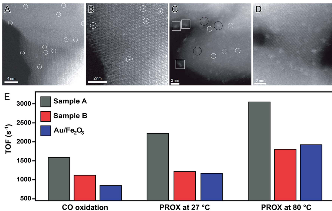
Fig. 6 Effect of NP size over catalytic activity. HAADF-STEM images of Pt single atoms (white circles) dispersed on \text{FeO}_x support obtained using a Pt/Fe atomic ratio of 1/1430 (0.17 wt% of Pt, (A and B)) and 1/95 (2.5 wt% of Pt, (C and D)). (E) Bar graph showing the turnover frequencies towards CO oxidation and PROX reaction at 27 and 80 °C employing \text{Pt}_1/\text{FeO}_x as catalysts. Commercial \text{Au/Fe}_2\text{O}_3 was also included for comparison. Adapted from ref. 92 with permission.
