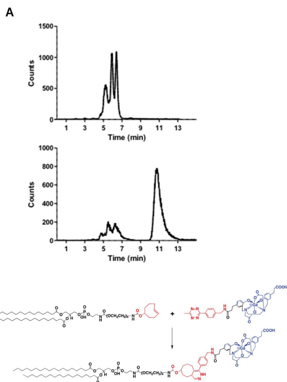
Fig. 4 (A) Radio-HPLC chromatograms of (top) ^{68}\text{Ga} -HBED-CC-tetrazine precursor and (bottom) reaction between 4 and 5, after 15 min at 60 ^{\circ}\text{C} . (B) Scheme of the reaction between TCO-modified PE (4) and ^{68}\text{Ga} -HBED-CC-tetrazine (5).
