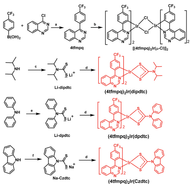
(a) Pd(PPh 3 ) 4 , Na 2 CO 3 , THF-H 2 O, 70 °C, 12h; (d) EtOCH 2 CH 2 OH, rt, 5 min; (b) IrCl 3 ·3H 2 O, EtOCH 2 CH 2 OH, 115 °C, 12h; (e) n -BuLi, CS 2 , 0 °C, 12h; (c) LiOH, CS 2 , benzene-H 2 O, rt, 2h; (f) NaH, CS 2 , 40 °C, 3h;
