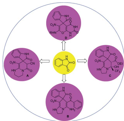
Fig. 2 Summary of previous works of spiropyridineoxindole synthesis.
