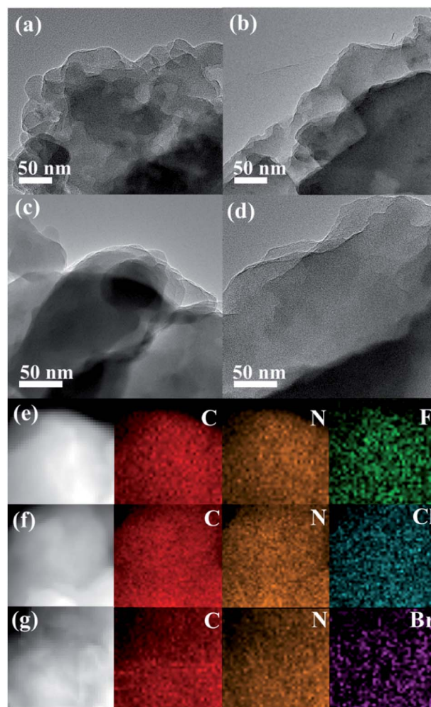
Fig. 1 TEM images of (a) CTF-1, (b) CTFE, (c) CTFCl and (d) CTFBr. EDX elemental mappings of (e) CTFE, (f) CTFCl and (g) CTFBr.
