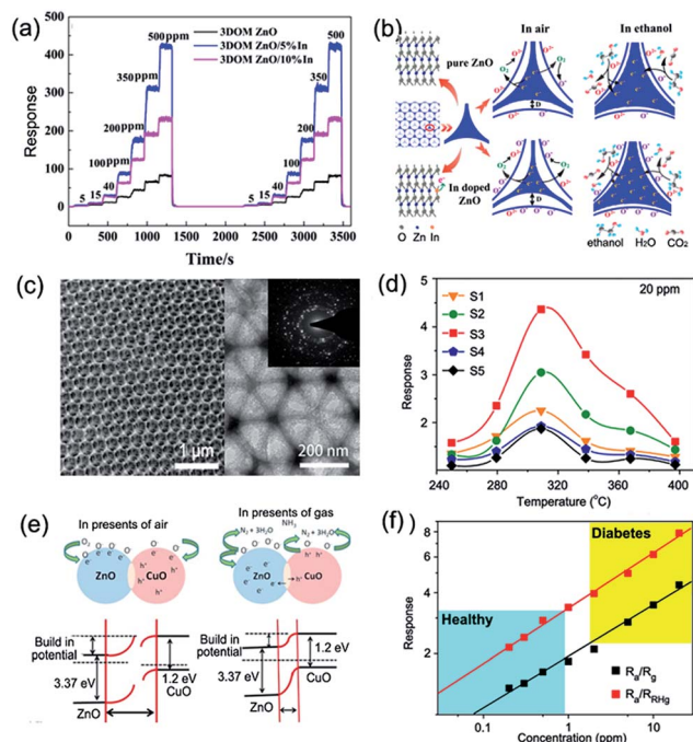
Fig. 11 (a) Dynamic response curves of typical 3DOM samples at different concentrations of ethanol at 250 °C. (b) Schematic diagram of ethanol sensing on the surface of pure and In-doped 3DOM ZnO. Reproduced with permission. 113 Copyright 2016, American Chemical Society. (c) Morphologies and microstructure of 3DOM ZnO–CuO arrays. (d) Acetone responses of S1–S5 ZnO–CuO 3DOM sensors as a function of the working temperature; here, Zn/Cu atomic ratios are 1 : 0, 3 : 1, 1 : 1, 1 : 3, and 0 : 1 and marked as samples S1–S5, respectively. (e) Schematic illustration of p–n-junction-enhanced sensing mechanism. (f) Response of S3 ZnO–CuO 3DOM sensor to very low acetone concentration under \sim 93.5\% RH. Reproduced with permission. 114 Copyright 2015, Elsevier Ltd.
