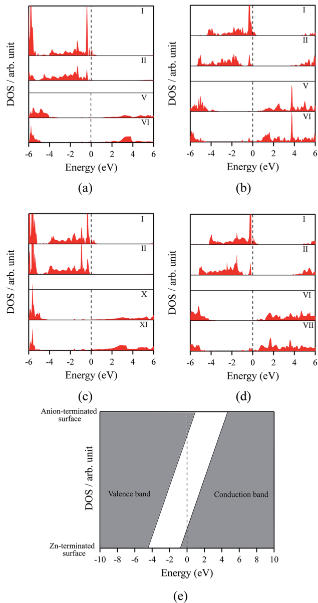
Fig. 6 Partial density of states (PDOS) per layer for polar ZnS(111) films with 6 layers for (a) ZnO and (b) ZnS. Partial density of states (PDOS) per layer for polar WZ(0001) films for (c) ZnO with 11 layers and (d) ZnS with 7 layers (the smallest thicknesses for which these structures are stable). The vertical dashed line indicates the Fermi level (e) Schematic band structure diagram of surface metallisation. A similar figure but expanded with PDOS plots for all the layers are given in the ESI.†
