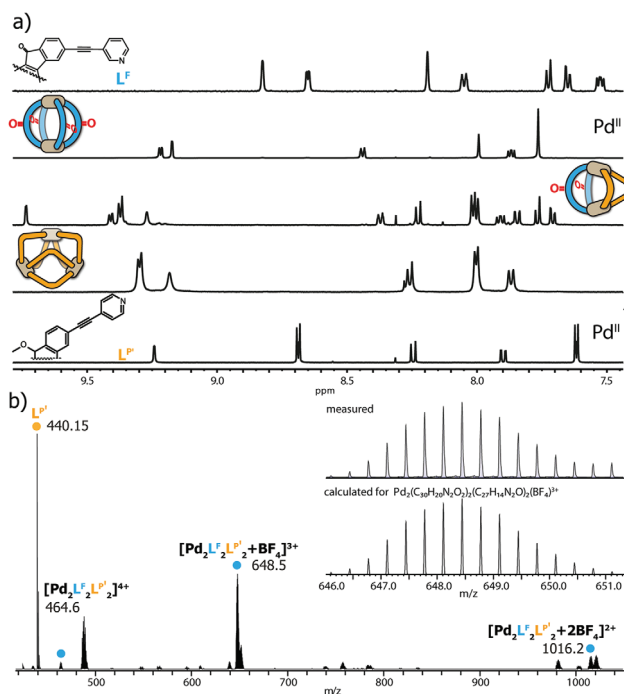
Fig. 2 (a) ^1H NMR spectra of L^F , homoleptic [Pd_2L^F_4]^{4+} , heteroleptic [Pd_2L^F_2L^P]^{4+} , homoleptic [Pd_3L^P_6]^{6+} and L^{P'} (from top to bottom, 500 MHz, 298 K, DMSO- d_6 ); (b) ESI mass spectrum of heteroleptic [Pd_2L^F_2L^{P'}]^{4+} , including BF_4^- adducts.
