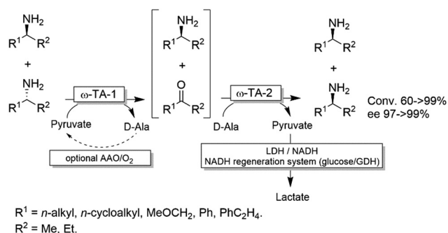
Scheme 18 One-pot deracemisation of amines using enantiocomplementary \omega -TAs in two temporally separated steps. LDH: Lactate dehydrogenase (EC 1.1.1.27), AAO: amino acid oxidase (EC 1.4.3.2), GDH: glucose dehydrogenase.
