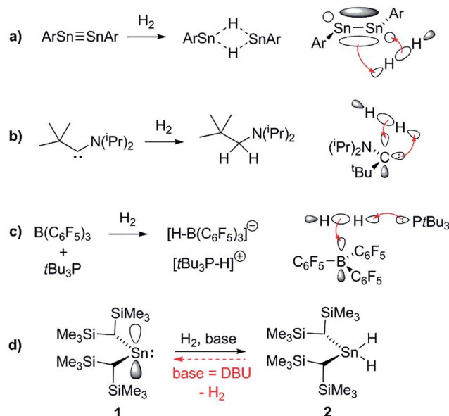
Fig. 1 Representative orbital interactions between H 2 and main group compounds: (a) unsaturated E–E compounds e.g. distannynes (Ar = C 6 H 2 -2,6-(C 6 H 3 -2,6- i Pr 2 ) 2 -4-X; X = H, SiMe 3 , F); for X = H, the reaction is reversible at 80 °C; 5a,13 (b) single site low-valent centres e.g. carbenes; 6a (c) sterically hindered LAs and LBs (FLPs); (d) this work.
