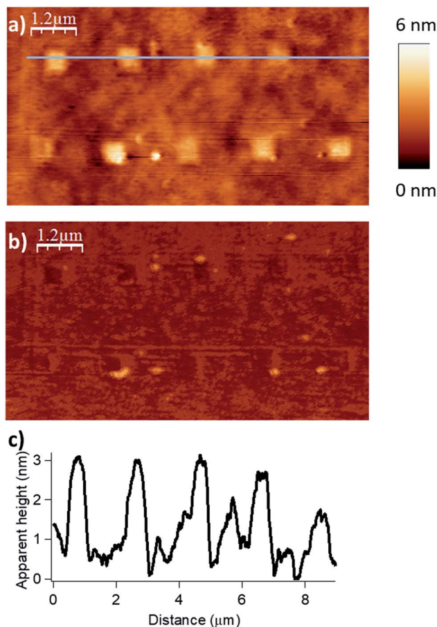
Fig. 2 Influence of the applied force ( F ) on the esterification reaction with myristic anhydride as acylating reagent ( D_{IL} = 8 nm, V_{scan} = 1 μm s -1 ). The applied force was incremented progressively from left to the right with respective values of 200, 1000, 2000, 2900 and 3800 nN for the upper line and 4800, 5700, 6700, 7600 and 9600 nN for the lower line. (a) Topography image in tapping mode after reaction. (b) Corresponding phase image. (c) Line profile (corresponding to the blue line in (a)) displaying an average height of 1.9–2.1 nm (theoretical calculated value of 1.78 nm in gas phase for a model, see Fig. S6 in the ESI†).
