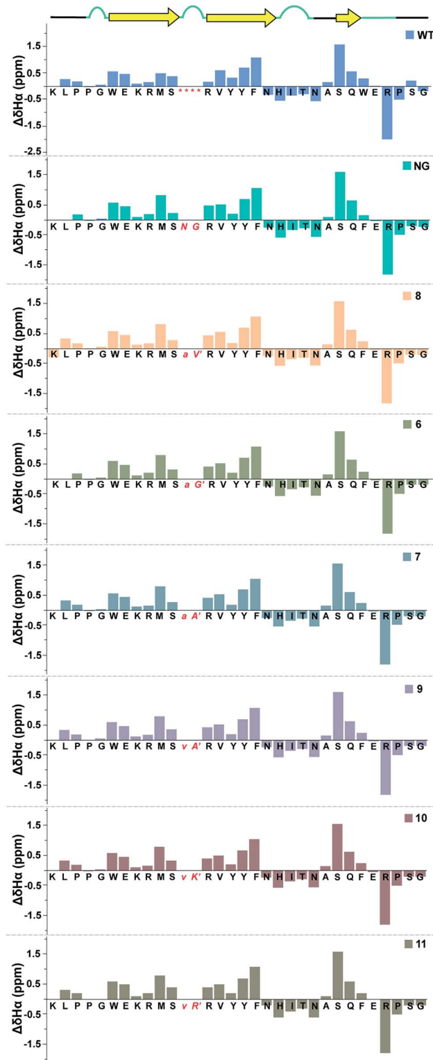
Fig. 7 Comparison of backbone H ^\alpha chemical shift deviation of the apo-Pin 1 WW domain (WT) with the \beta' turn (NG) and the re-engineered Pin 1 variants deduced from the predicted random coil values, ^{37} indicating minimal perturbation in the secondary structure. The -\text{RSSG}- motif in loop 1 of WT is indicated by an asterisk.
