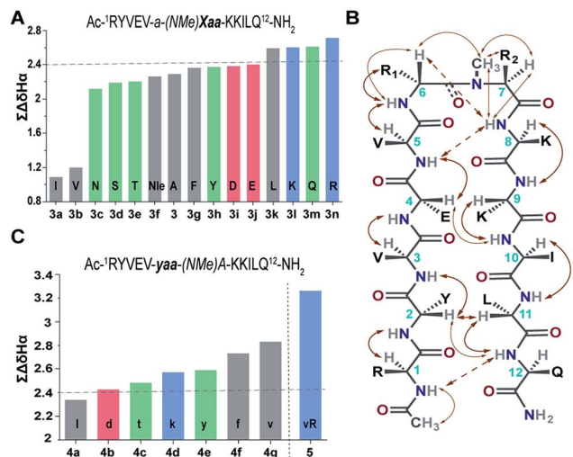
Fig. 4 (A) \Sigma\text{CSD} of the primary library with L-amino acid substitutions (Xaa) at the i +2 site. (B) The characteristic NOEs, where the thick arrows denote strong (1.8–2.1 Å), the thin arrows denote medium (2.2–2.5 Å) and the broken arrows denote weak (>2.6 Å) NOEs. (C) \Sigma\text{CSD} of the secondary library with i +1 substitutions (yaa) along with 5 derived from the combination of 4g and 3n. All the NMR measurements were done in acetate buffer (pH 3.8) at 25 °C.
