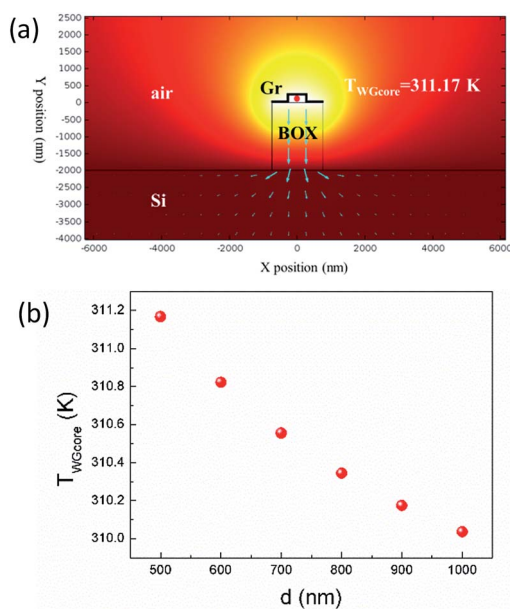
Fig. 6 (a) Thermal field distribution with 1.94 \mu\text{m} -wide graphene nanoheater. Blue arrows shows directions of heat flux. (b) Waveguide core temperature as function of d .
