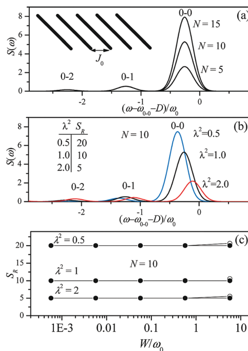
Fig. 1 Changes in the fluorescence spectra as a function of (a) the number of subunits N and (b) Huang-Rhys factor \lambda^2 . Exciton bandwidth is set W = \omega_0 = 1400 \text{ cm}^{-1} in (a) and (b). (c) Fluorescence vibronic peak ratio S_R as a function of exciton bandwidth. Adapted from ref. 8 with permission. Copyright 2011 American Chemical Society.
