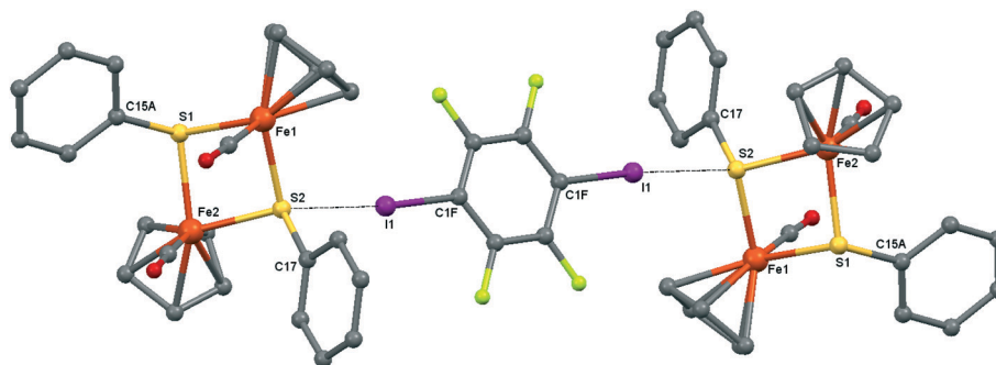
Fig. 4 Crystal structure diagram of 2 , showing its I–S halogen-bonded trimolecular assemblies ([\text{CpFe}(\text{CO})_2(\mu_2\text{-SPh})_2(\mu_2\text{-DITFB})])_n . Hydrogen atoms are omitted for clarity. Selected distances (Å): I(1)–S(2), 3.130(1). Selected angles (°): C(1F)–I(1)–S(2), 173.9(1); Fe(1)–S(2)–I(1), 111.91(4); I(1)–S(2)–C(17), 102.5(1); I(1)–S(2)–Fe(2), 118.86(4). Dotted lines link S and I atoms at a distance shorter than the sum of the S–I vdW radii. 18
