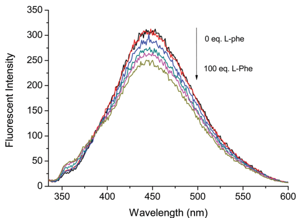
Fig. 4 Fluorescence based titrations of NI-cho1 (10 \mu\text{M} ) in \text{CH}_3\text{CN} -DMSO (95 : 5, v/v) with various equivalents of Boc-L-Phe.
