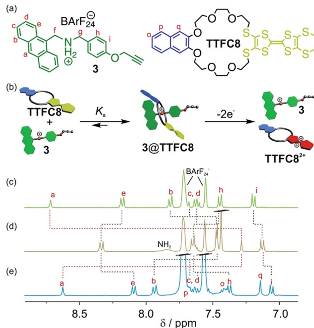
Fig. 2 (a) Structures of macrocycle TTCF8 and ammonium axle 3 . (b) Schematic representation of the association between ammonium axle 3 and macrocycle TTCF8 and the axle expulsion induced by double oxidation of the macrocycle. Stacked partial ^1\text{H} NMR spectra (400 MHz, 2 mM, \text{CD}_2\text{Cl}_2 , 298 K) of (c) ammonium axle 3 , (d) pseudo[2]rotaxane 3@TTCF8 and (e) after oxidation by two equiv. of \text{Fe}(\text{ClO}_4)_3 and addition of 5 equiv. tetrabutylammonium \text{BArF}_{24}^- as stabilising electrolyte.
