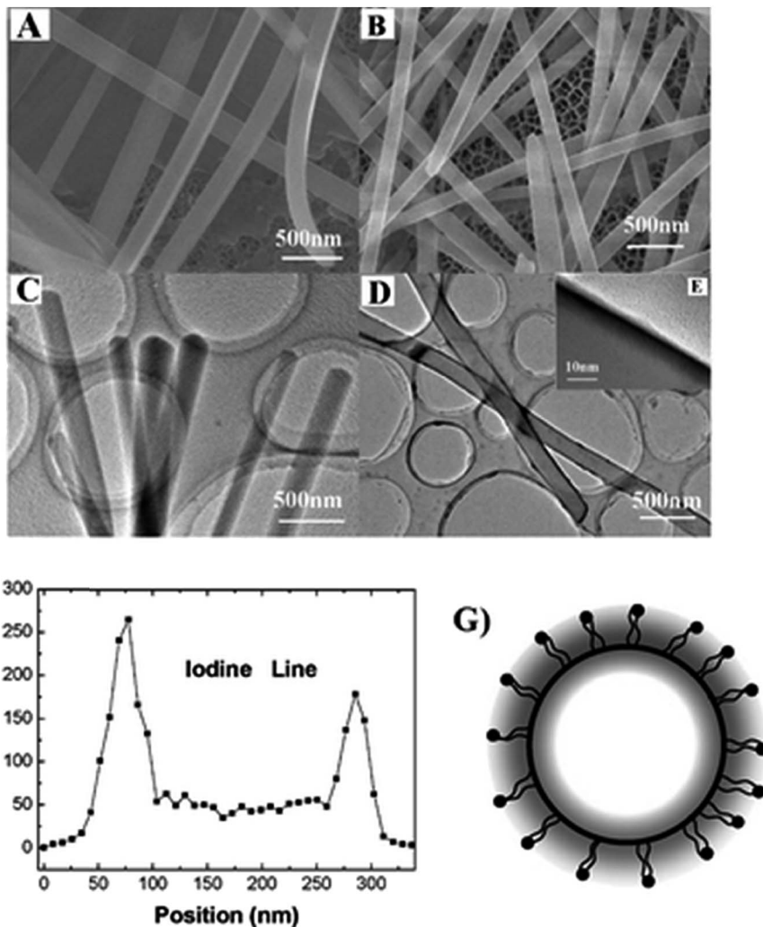
Fig. 11 (A) SEM and (C) TEM images of the pristine nanorods of DPNP; (B) SEM and (D) low-magnification TEM and (E) high magnification TEM images of DPNP/dye 1 core/diffuse-shell nanorods; (F) HRTEM-assisted EDS line of elemental iodine analysis across the section of a single core/diffuse-shell nanorod. (G) Schematic illustration of the section of the core/diffuse-shell nanorod. Scale bars: (A–D) 500 nm; (E) 10 nm. Reproduced from ref. 161 with the permission from The Royal Society of Chemistry.
