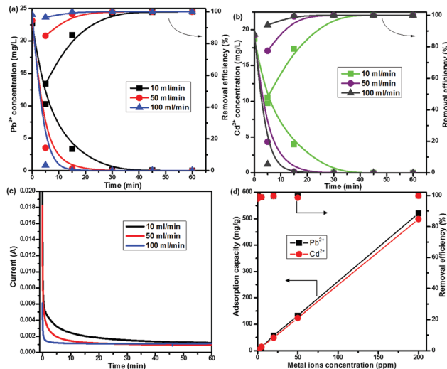
Fig. 2 MCDI performance for (a) Pb^{2+} and (b) Cd^{2+} removal at different flow rates; (c) the corresponding I-t curves; and (d) removal efficiency and adsorption capacity of Pb^{2+} and Cd^{2+} at different concentrations (0.05–200 ppm, flow rate: 50 \text{ ml min}^{-1} , 25 mg materials, 50 ml solution, 1.2 V, batch mode).
