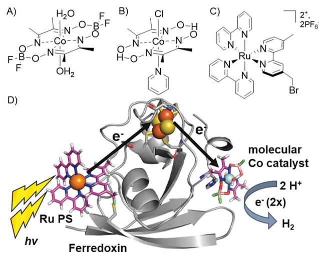
Fig. 1 (A–C) Catalysts and photosensitizers used in the current study. Cobaloxime catalysts (A) \text{Co}(\text{dmgBF}_2)_2 \cdot 2\text{H}_2\text{O} ( \text{CoBF}_2 ) and (B) [\text{Co}(\text{dmgH})_2\text{pyridyl}]\text{Cl} ( \text{CoPy} ) and (C) ruthenium photosensitizer (Ru PS), [\text{Ru}(4\text{-CH}_2\text{Br-4'-CH}_3\text{-2,2'-bpy})(\text{bpy})_2] \cdot 2\text{PF}_6 . (D) Photocatalytic hydrogen production scheme in Ru-Fd- \text{CoBF}_2 biohybrid utilizing electron transfer through the native Fd [2\text{Fe-2S}] cluster (1A70). 25
