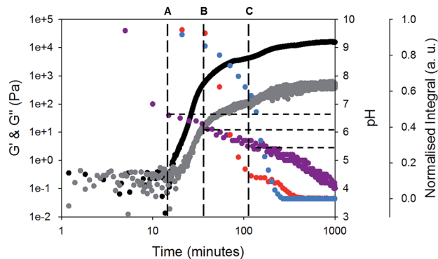
Fig. 3 Monitoring gelation of 1 and 2 over time. The change in intensity of peaks from 1 H NMR spectroscopy during gelation of the CH 3 peak at 1.70 ppm from gelator-1 (blue) and the CH 2 at 3.05 ppm from gelator-2 (red) are compared to change in pH during gelation of 1 and 2 (purple). The change in G' and G'' over time for gel-1,2 is also shown (black data are G' and grey data are G'' ), rheological time sweeps were performed at a strain of 0.5%, 10 \text{ rad s}^{-1} and at 25 \text{ }^\circ\text{C} . For discussion around points A, B, and C, please see main text.
