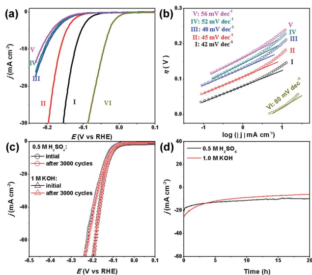
Fig. 5 (a) Polarization curves and (b) Tafel plots for the HER on modified GCEs comprising (I) MoC–Mo 2 C-31.4, (II) Mo 2 C, (III) MoC–Mo 2 C-68.1, (IV) MoC–Mo 2 C-30 (mixed), (V) MoC, and (VI) commercial Pt/C in 1.0 M KOH. (c) Stability of the MoC/Mo 2 C-31.4 modified electrodes with an initial polarization curve and after 3000 cycles in 0.5 M H 2 SO 4 and 1.0 M KOH, and (d) the long-term durability tests at \eta = 190 mV.
