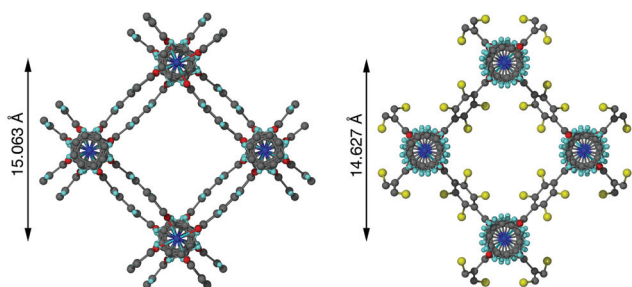
Fig. 1 Pore structure of [\text{Zn}_2(\text{bdc})_2(\text{dabco})] \cdot 4\text{DMF} \cdot 0.5\text{H}_2\text{O} (left) and [\text{Zn}_2(\text{bdc-Br})_2(\text{dabco})] (right), the latter showing a slight diagonal compression of the pore with the addition of bromine substituents into the framework. The bromine atom in [\text{Zn}_2(\text{bdc-Br})_2(\text{dabco})] is disordered over four positions.
