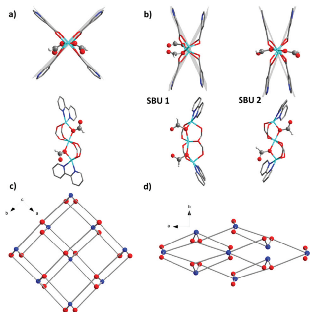
Fig. 4 (a) SBU 1 of 1; (b) SBU 1 and SBU 2 of 1'; (c) crystal structure of 1; (d) crystal structure of 1'. (Colour code in (c) and (d): blue spheres – SBU units, and red spheres – \text{bpydc}^{2-} linkers).
