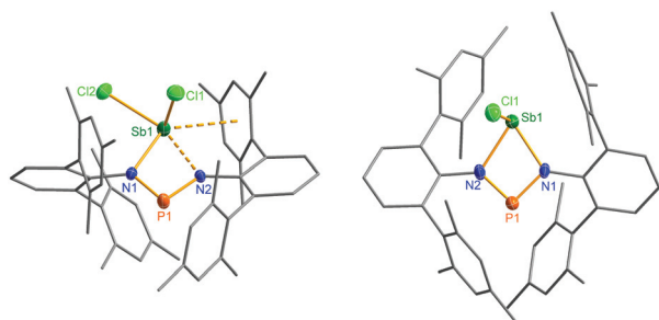
Fig. 6 Molecular structure of 2a (left) and 3 (right). Thermal ellipsoids are drawn at 50% probability (173 K). Selected bond lengths [Å] and angles [°]: 2 : Sb1–N1 2.133(4), Sb1–N2 2.392(4), Sb1–Cl1 2.358(2), Sb1–Cl2 2.451(2), P1–N1 1.623(4), P1–N2 1.598(4), N2–P1–N1 96.0(2). 3 : Sb1–N1 2.136(3), Sb1–N2 2.171(3), Sb1–Cl1 2.342(1), P1–N2 1.625(3), P1–N1 1.643(4), N2–P1–N1 91.7(2).
