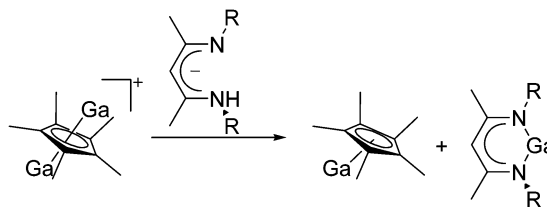
Fig. 16 The [\text{Ga}_2(\eta^5\text{-Cp}^*)]^+[\text{B}(\text{Ar}^{\text{CF}_3})_4]^- salt cleanly reacts as a gallium(i) source with ligands such as \text{DDP} .
