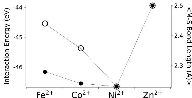
Fig. 2 The calculated interaction energy and bond length between metal ions and methanethiolates. Associated plots of charge and force constants can be found in Fig. S7 (ESI † ). Filled circles represent average metal–sulphur bond lengths, while open circles represent interaction energies in the gas phase.
