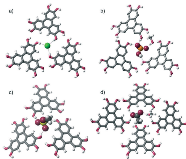
Fig. 2 Comparison of the anion environments in solid state structures of [HHTP·TBA·X] n : a) [HHTP·TBA·Cl] n (the anion environments in [HHTP·TBA·I] n and [HHTP·TEA·Cl] n are very similar); b) [HHTP·TBA·H 2 PO 4 ] n ; c) [HHTP·TBA·MeOSO 3 ] n ; d) [HHTP·TBA·OAc] n .
