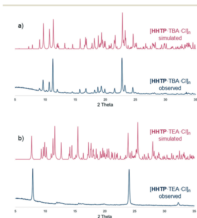
Fig. 3 PXRD traces of dried, bulk samples of a) [\text{HHTP} \cdot \text{TBA} \cdot \text{Cl}]_n and b) [\text{HHTP} \cdot \text{TEA} \cdot \text{Cl}]_n as well as traces simulated from SCXRD data (see ESI† for full details).
