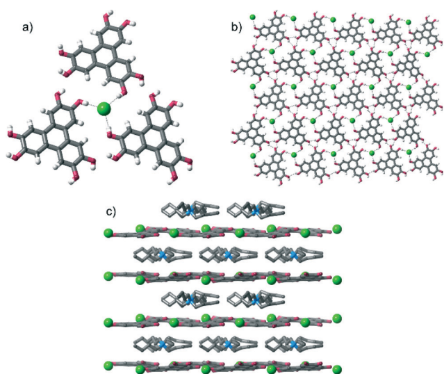
Fig. 1 Views of the solid state structure of [HHTP·TBA-Cl] n : a) environment around Cl - anion; b) 2D sheet formed from HHTP molecules and anions; c) packing viewed along c axis (with hydrogen atoms omitted for clarity). TBA cation disorder is omitted for clarity.
