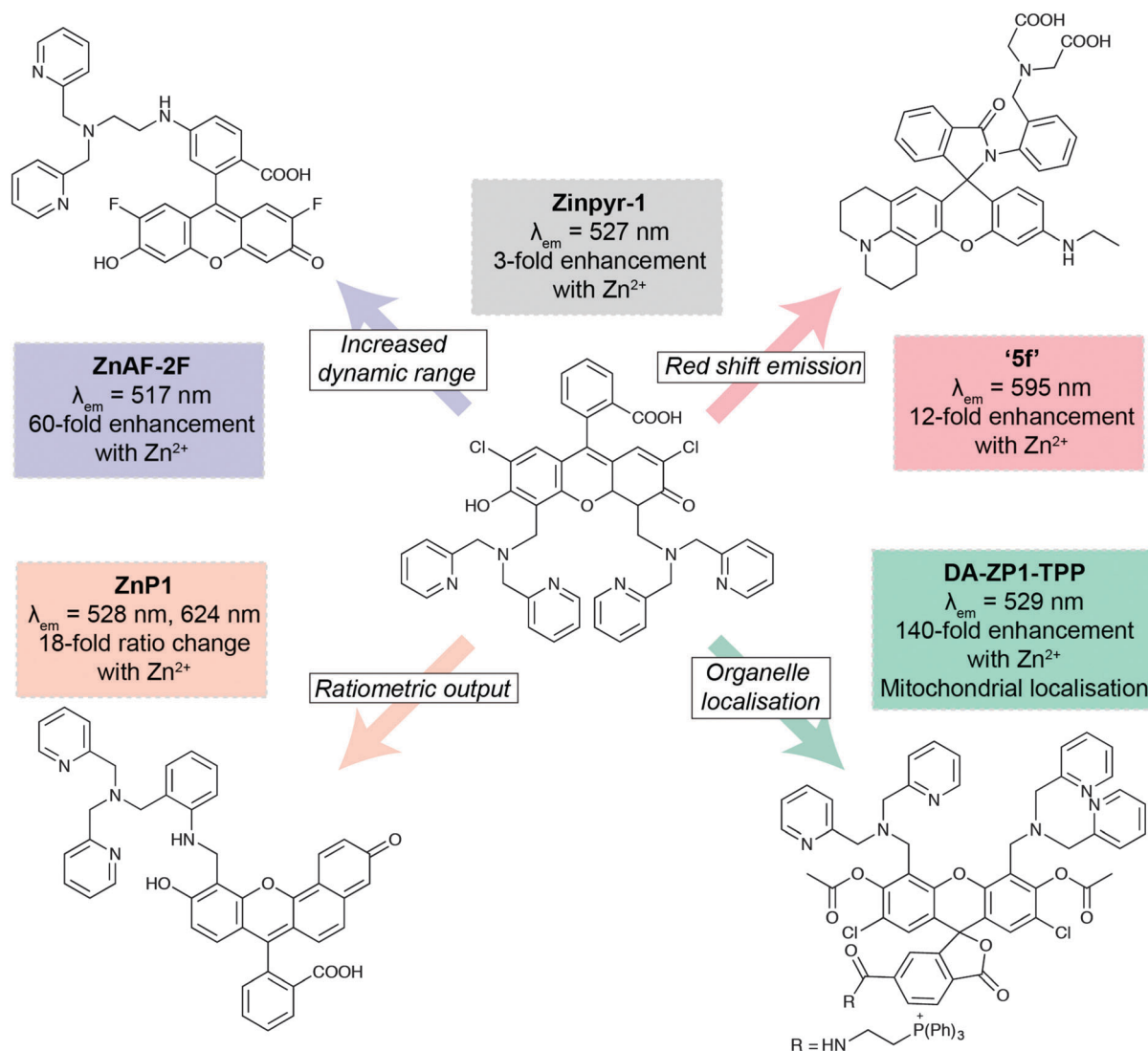
Fig. 6 Key developments in xanthene-based fluorescent sensors for \text{Zn}^{2+} . Zinpyr-1 98 has been further developed to improve than range of \text{Zn}^{2+} concentrations it can detect ( ZnAF-2F ), 99 measure \text{Zn}^{2+} flux via ratiometric measurements ( ZnP1 ), 100 localise within specific organelles, such as mitochondria ( DA-ZP1-TPP ), 101 and optimise its fluorescence emission peak ( 5f ). 102
