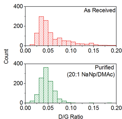
Fig. 7 Distribution of D/G Raman ratios of Elicarb SWCNTs before and after NaNp purification ( 20 : 1 purification, 633 nm excitation). D/G of as received SWCNTs = 0.06 \pm 0.037 , D/G of as purified SWCNTs = 0.047 \pm 0.015 .
