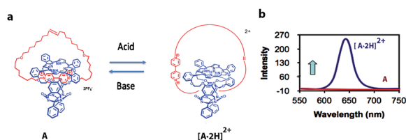
Fig. 2 (a) Acid-driven switching of porphyrin[2]catenane A . 21 (b) Fluorescence spectra of [2]catenanes A (red) and [\mathbf{A} \cdot 2\text{H}]^{2+} (blue).
