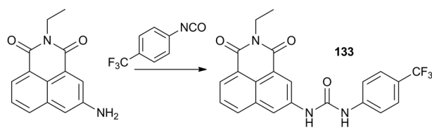
Scheme 15 Synthesis of anion sensor 133 .
